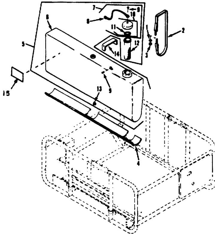
Figure 11. Fuel tank.
