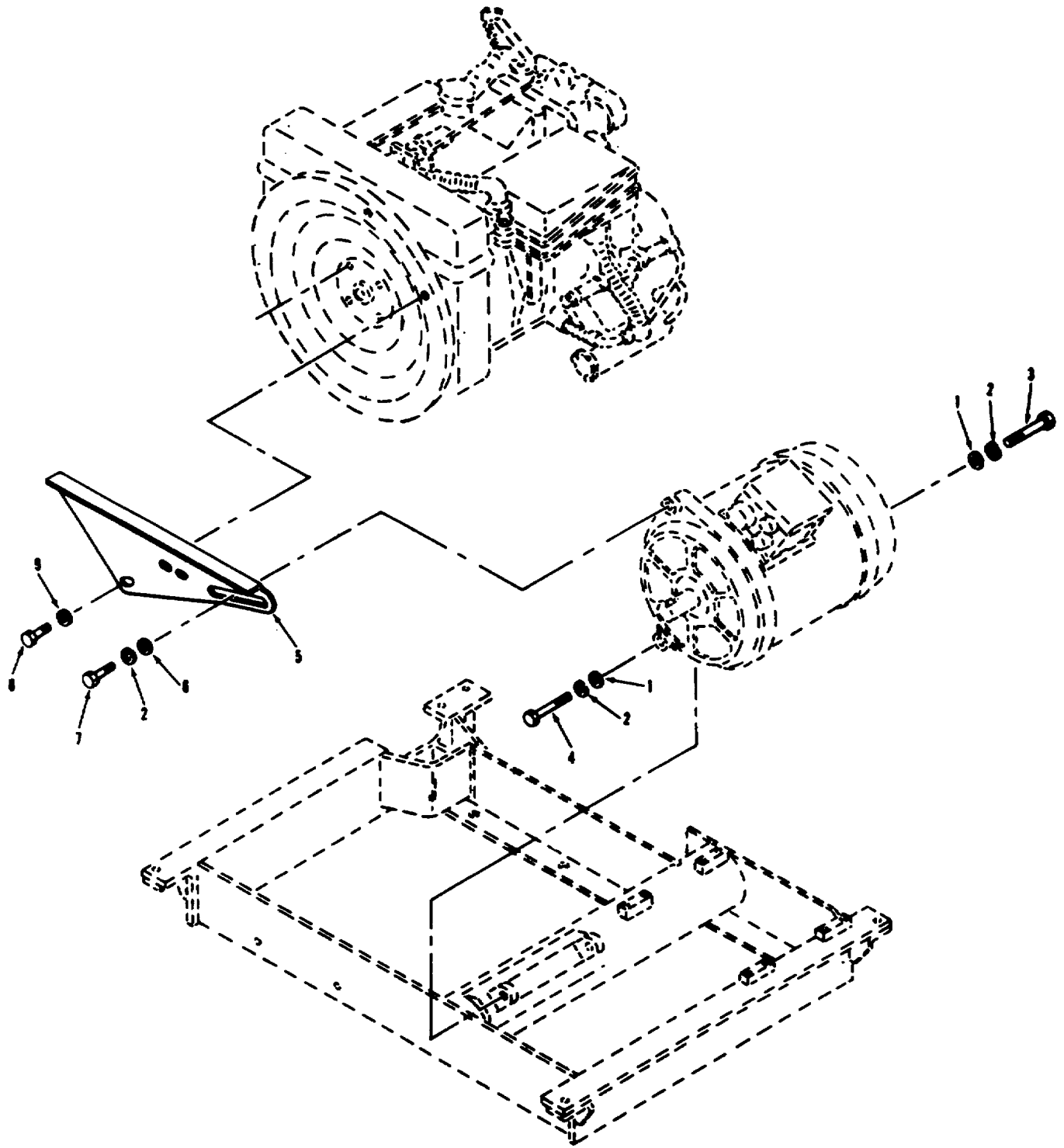
Figure 12. Generator mounting.
