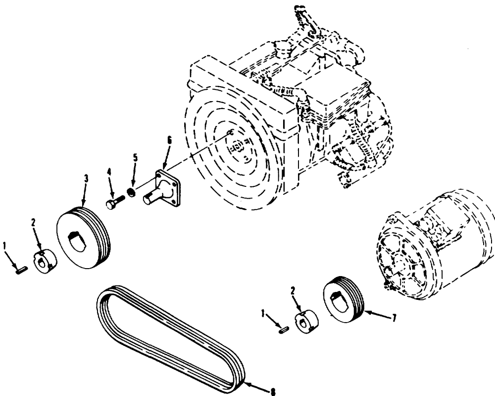
Figure 7. Drive belts.
