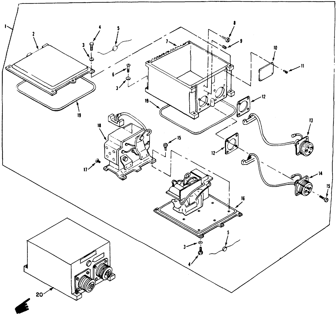
Figure 10. Generator regulator.
